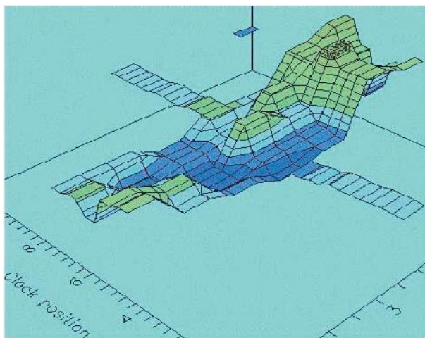
Figure 2. FSM monitoring software produces graphical plots that indicate the location and severity of defects and also calculates corrosion rates.
